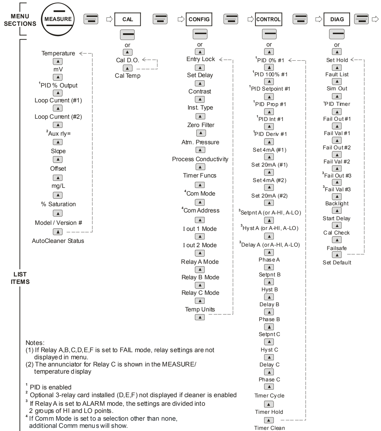
Figure 16 - Software Map
