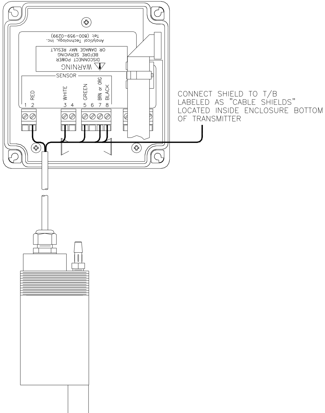
Figure 14 - Sensor Wiring
