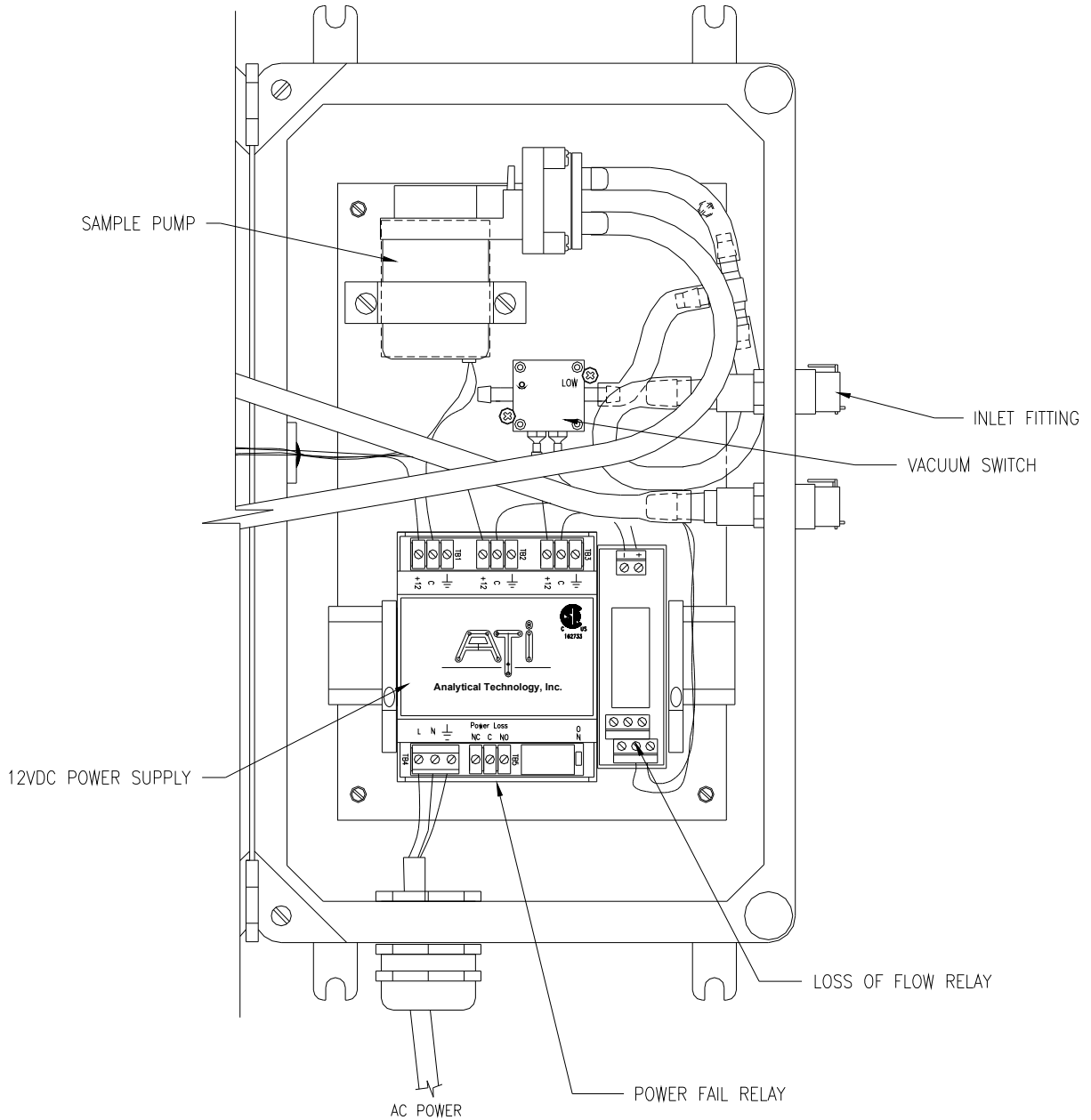
Figure 3 - Power and alarm output connections 120 VAC version (ATI-0230)
