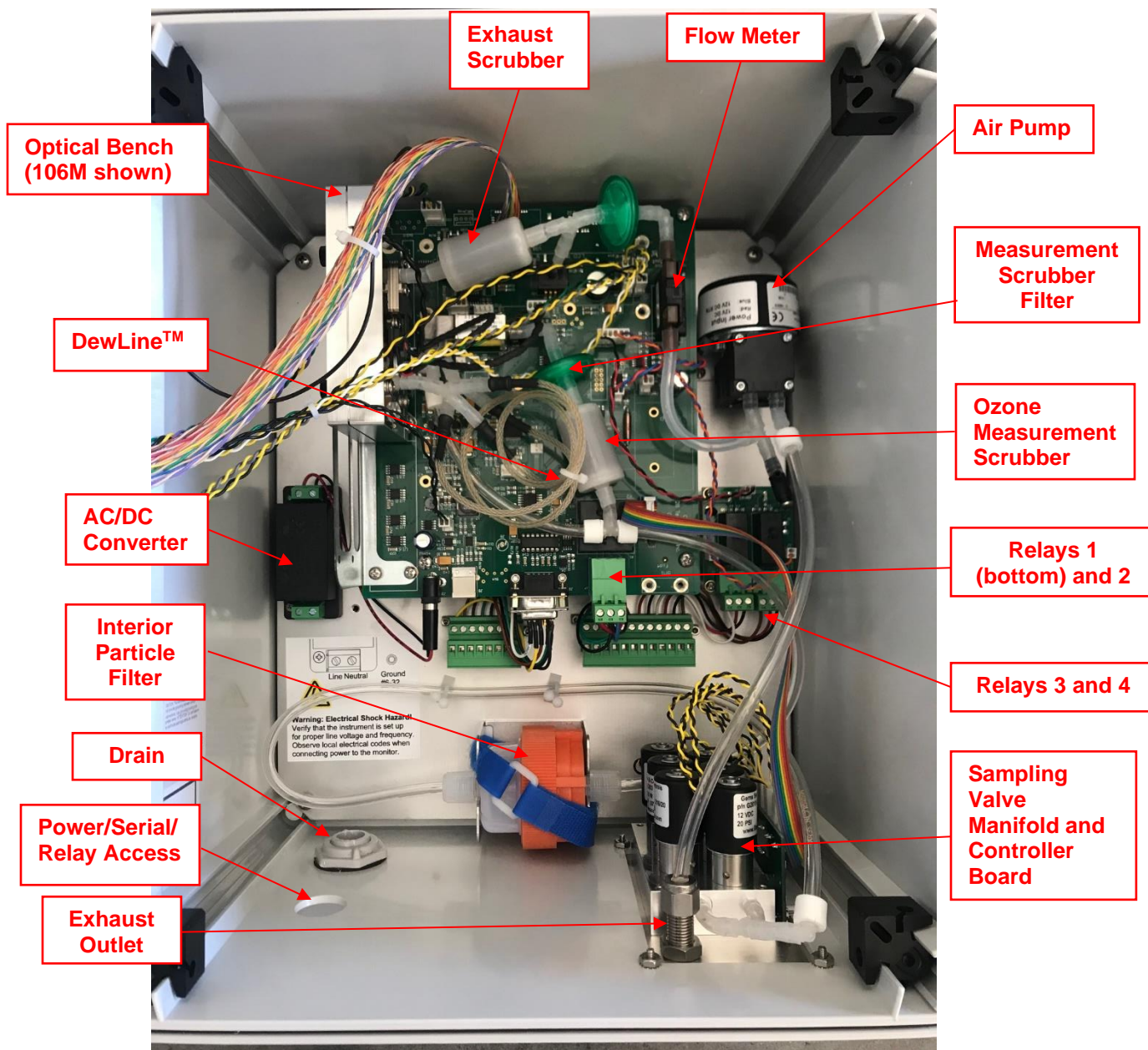
Figure D-8. Top inside view. The 106-M is shown, which has a shorter optical bench than the 106-L.
