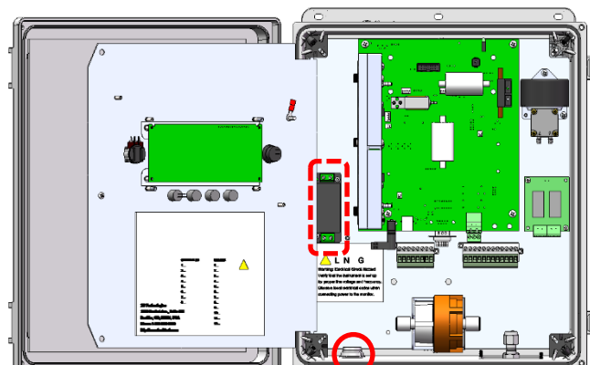
Figure D-3. Instrument layout and power points.
