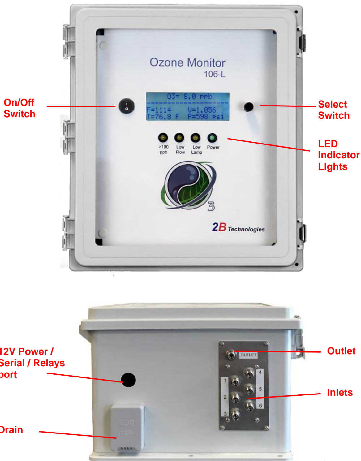
Figure D-6. Front and bottom views of the Model 106-L-MC6 Multi-channel Ozone Monitor.
