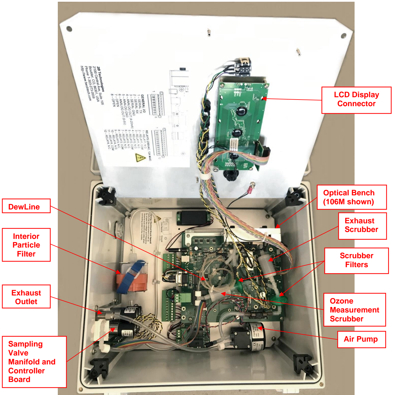
Figure D-7. Full open view of the Model 106-M-MC6 Ozone Monitor. The 106-L-MC6 has a longer optical bench but is otherwise similar. See Figures 7.1a and 7.1b of this manual for a better view of the analogous components.
